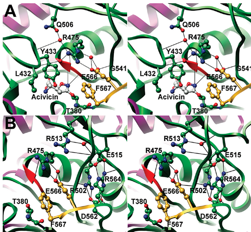
FIGURE 7: An extensive hydrogen bond network in the C-terminal region of the 20 kDa subunit of HpGT is required for autoprocessing and catalytic activity. In the stereo diagrams, a ribbon illustration of HpGT is presented with relevant residues shown in ball and stick representation. Atoms are colored as in Figure 4, and potential hydrogen bonds were identified with Chimera (indicated as solid black lines). Gly 472 and Gly 473, whose backbone amides form the proposed oxyanion hole, are highlighted as a red ribbon. (A) Arg 475 is critical for positioning of both the Tyr 433 loop and the Phe 567 C-terminal tail, as well as the backbone amides of Gly 472 and Gly 473. (B) The Glu 515/Arg 564 and the Asp 562/Arg 502 salt bridges stabilize the active site region and are critical for autoprocessing and enzymatic activity. Arg 513 also contributes to the overall integrity of the active site.
