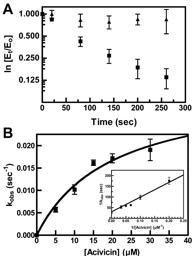
FIGURE 2: Inactivation of HpGT by acivicin. (A) HpGT (0.1 mg/mL) was incubated with 10 \mu M acivicin at pH 7.4 and 4 °C in the absence (squares) and presence (triangles) of 1 mM glutamate. The k_{obs} for the reactions was determined from the slope of \ln(E_t/E_0) versus time, where E_0 and E_t are the enzymatic activities at time 0 and time t , respectively. (B) Dependence of the rate of HpGT inactivation on acivicin concentration. HpGT was incubated with various concentrations of acivicin and the rate of inactivation determined as in panel A. (Inset) Double reciprocal plot used to calculate k_{max} and K_i .
