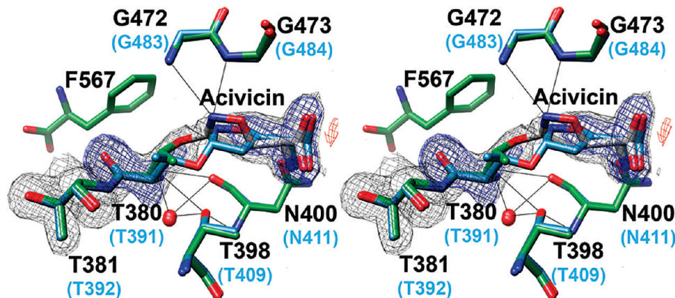
FIGURE 3: Electron density corresponding to the site of acivicin modification. The refined model of acivicin-modified HpGT with pertinent active site residues is shown in stick representation and is superimposed with acivicin-modified E. coli \gamma GT. Oxygen atoms are shown in red and nitrogen atoms in blue. Carbon atoms are colored green in HpGT, gray in acivicin, and blue in E. coli \gamma GT. Residue numbers are noted in black (HpGT) and blue ( E. coli \gamma GT). Also shown are the calculated electron density maps after the initial round of refinement, prior to inclusion of Thr 380 and acivicin in the model. The relevant 2F_o - F_c electron density is contoured at 1.0\sigma and illustrated in black. Positive and negative peaks in the difference map, contoured at 3.0\sigma , are shown in blue and red, respectively. Potential hydrogen bonds were identified with Chimera and are indicated as solid black lines.
