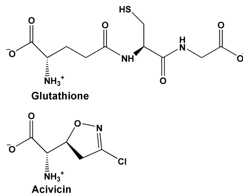
FIGURE 1: Comparison of glutathione and acivicin structures.
