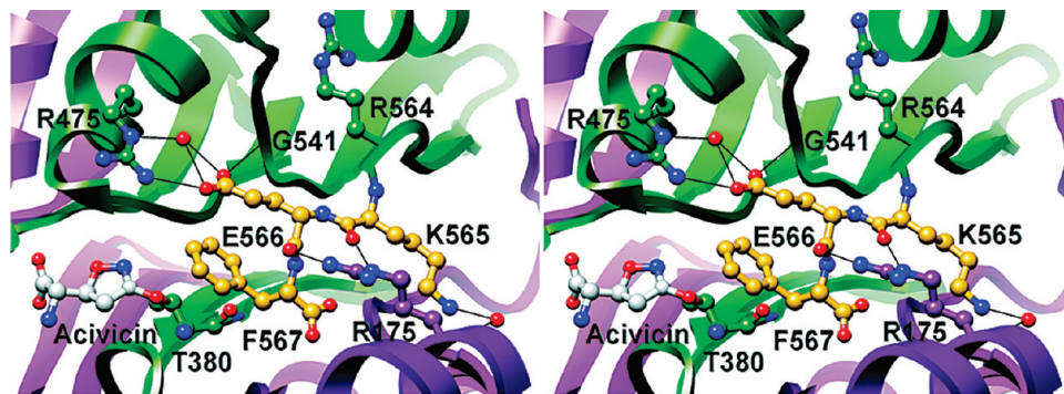
FIGURE 5: The C-terminus is ordered in the acivicin-modified HpGT structure. A ribbon stereo diagram of HpGT is shown with the 40 kDa subunit colored in purple and the 20 kDa subunit in green. Relevant active site residues are shown in ball and stick representation. Carbon atoms are colored in green (20 kDa subunit), purple (40 kDa subunit), gray (acivicin), and yellow (the ordered C-terminus). Oxygen atoms are shown in red and nitrogen atoms in blue. In each of the previously determined HpGT structures, residues Lys 565, Glu 566, and Phe 567 were disordered. In the acivicin-modified HpGT structure, unambiguous electron density corresponding to the C-terminus of the protein was observed (not shown). Residues Arg 175 and Arg 475 appear to stabilize this region, positioning Phe 567 over the catalytic nucleophile, Thr 380.
