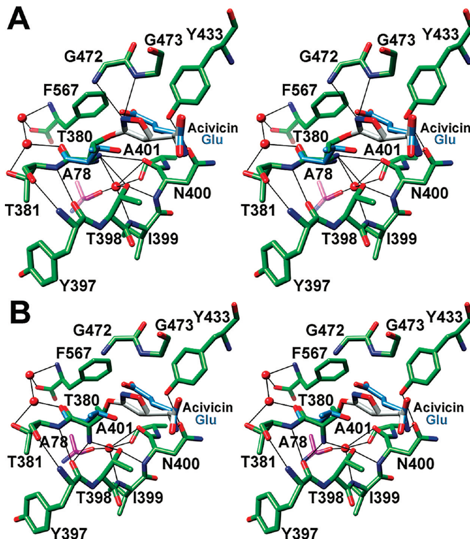
FIGURE 4: Alternate conformations of Thr 380 following acivicin modification. Crystals of acivicin-modified HpGT contain a heterotetramer within the asymmetric unit and provide two separate active site models. The active site regions of the refined structure are colored as in Figure 3. For reference, Thr 380 and bound glutamate from the previously determined HpGT–glutamate complex (blue) have been superimposed (20). The dihydroisoxazole ring of acivicin superimposes reasonably well with the glutamate side chain, and nearly identical placements of active site residues are observed with the exception of the slight displacement of Thr 380. (A) Within one active site, formed by the A and B subunits of the heterotetramer, Thr 380 adopts a conformation comparable to previous HpGT structures, with its \alpha -amino group within hydrogen bond distance to the backbone carbonyl group of Asn 400, the hydroxyl group of Thr 398, and a tightly bound water molecule. (B) In the second active site comprised of subunits C and D, Thr 380 has rotated such that its \alpha -amino group is within hydrogen bond distance to the backbone carbonyl group of Tyr 397 and the hydroxyl group of Thr 398. A nearly identical placement of acivicin is observed in both active sites.
